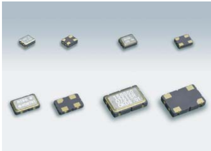
Actual size DSO221SR DSO321SR DSO531SR DSO751SR
