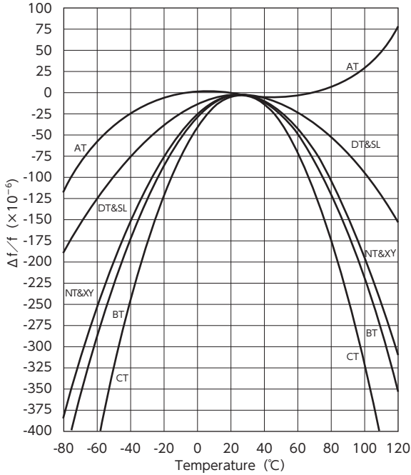
Temperature Characteristics for Various Cuts
