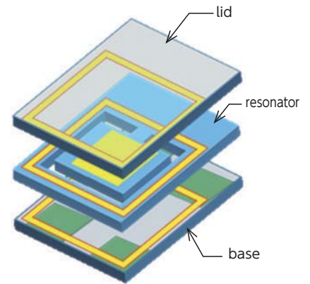
Fig.1 Structure of the Arkh.3G
