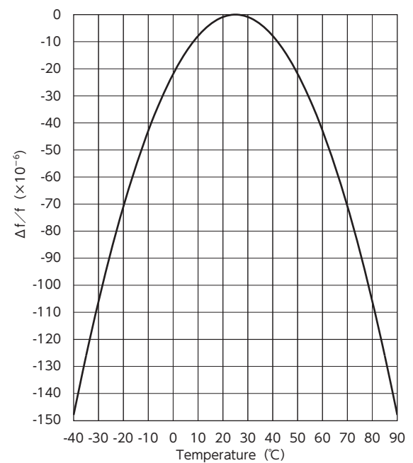
Temperature Characteristics for Tuning Fork Crystal Resonator
