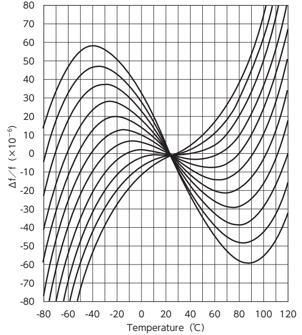
Temperature Characteristics for AT Cuts
