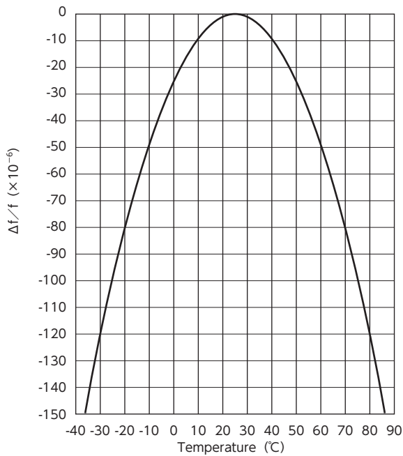
Temperature Characteristics for BT Cuts
