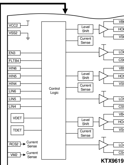
3-phase BLDC Motor Controller for 6-wire 3 Full-Bridges 100V Gate Driver Adjustable Over-current Protection Built-in charge pump with 96% duty cycle support 0.3A Source and 1.3A Sink Gate Driver Current Capability QFN77-56 Package
