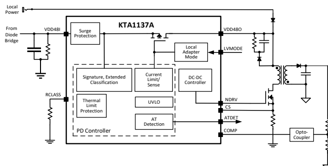
13W/30W PoE PD and DC-DC Controller IEEE 802.3af/at/bt Type 1 & 2 Compliant Internal 100V Hot-Swap Switch Type 2 PSE Detect, Local Power Capable 5 x 5mm QFN55-20
