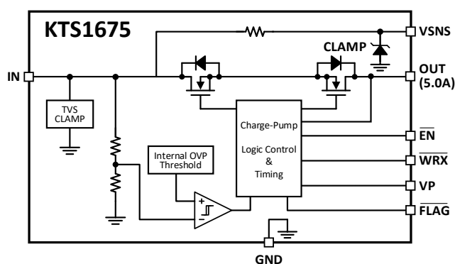
5.0A, \pm 100V Surge, VP Selectable OVP Switch with RBP
