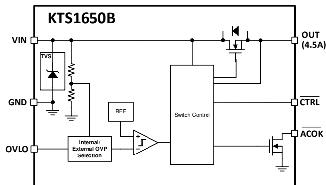
4.5A, \pm 200V Surge, 24V Fixed or Adjustable OVP Switch
