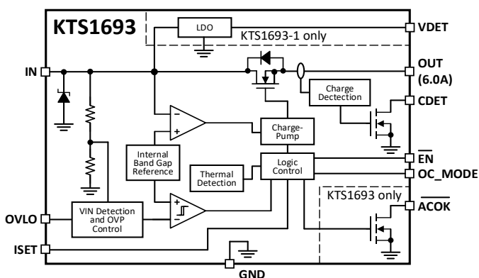
6A, \pm 110V Surge, 28V Fixed or Adjustable OVP with OCP, CL, CDET, ACOK
