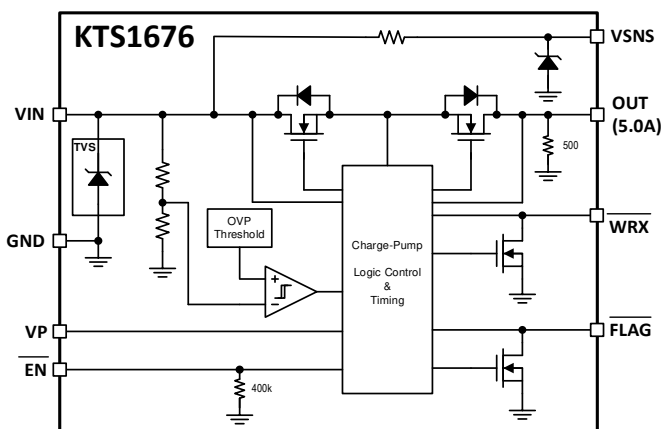
5.0A, \pm 100V Surge, Selectable OVP Switch with RBP
