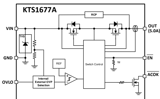
5A, \pm 90V Surge, 30V OVP Switch with RBP and SCP V_{IN} : 3V – 30V; I_{OUT} = 5.0A, R_{ON} = 30m \Omega , OVP Adj: 4V – 23V; Fixed: 23V
