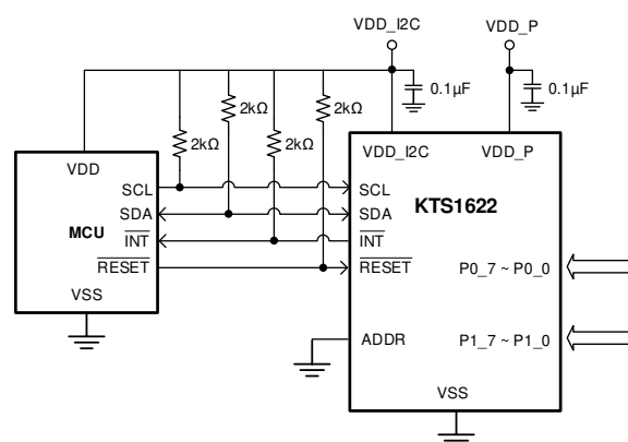
Low Voltage 16-bit I²C I/O Expander
